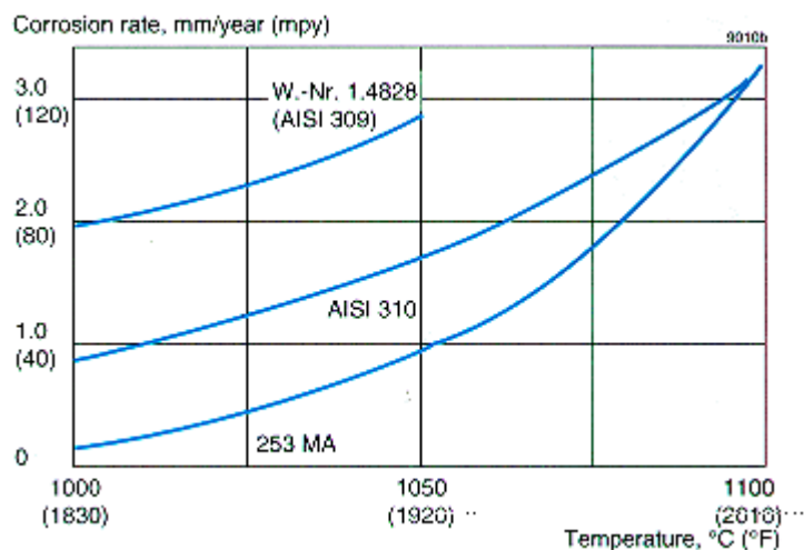
Figure 4. Oxidation in air during 1000 h cyclic exposure. The cycles comprise 15 min. at the testing temperature and 5 min. at room temperature. The curves represent averages.
