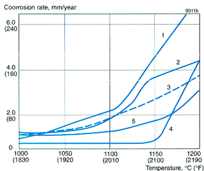
Figure 3. Oxidation in air during cyclic testing 5x24 h with cooling to room temperature every 24 h. Comparison of Sandvik 253 MA with four other high temperature materials.
